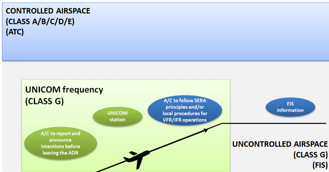
Figure 14: Departure IFR traffic in an aerodrome with non-ATS aeronautical stations: UNICOM (profile view)
