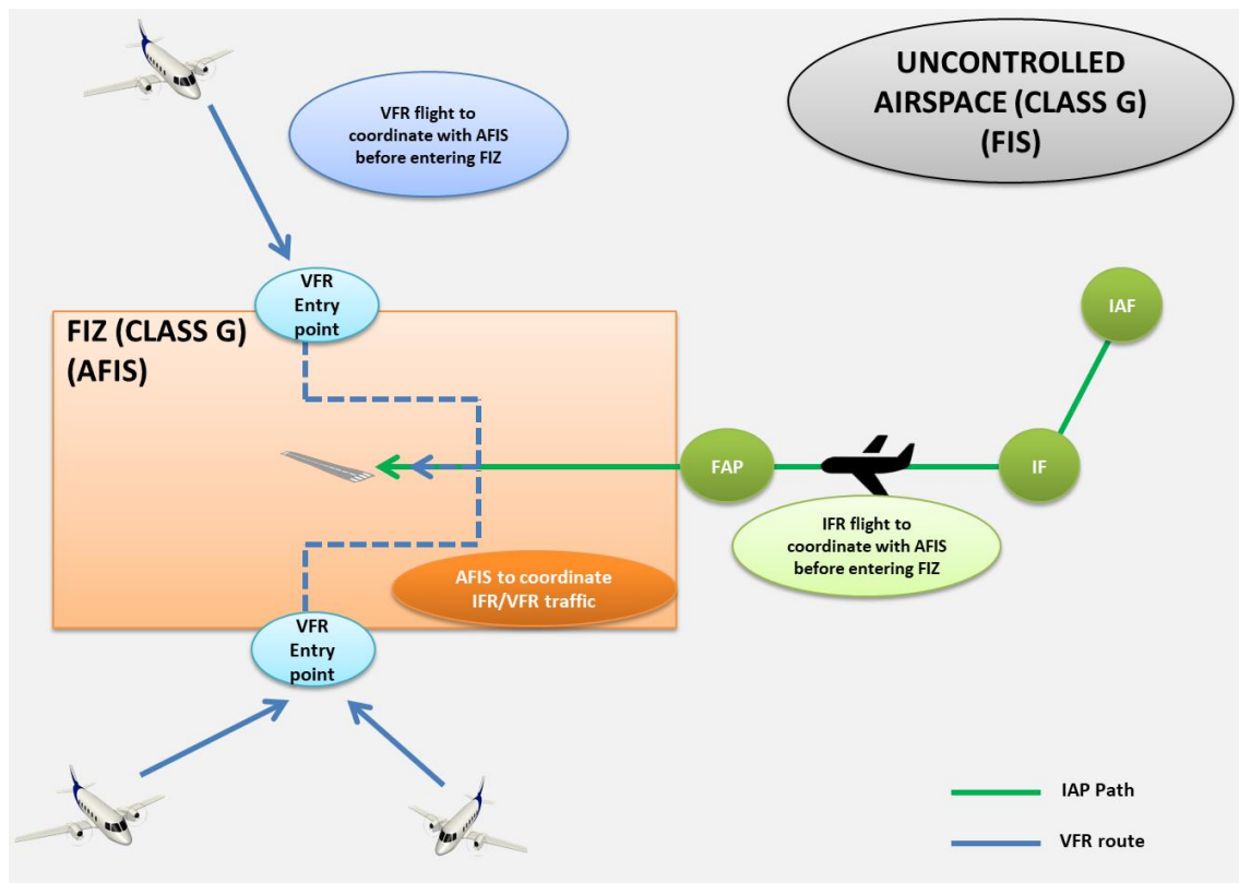
Figure 12: IFR/VFR integration within FIZ – AFIS service (plan view)
