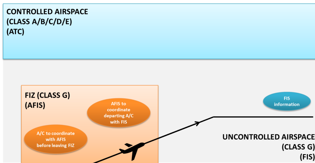
Figure 11: Departure IFR traffic with AFIS (vertical view)
