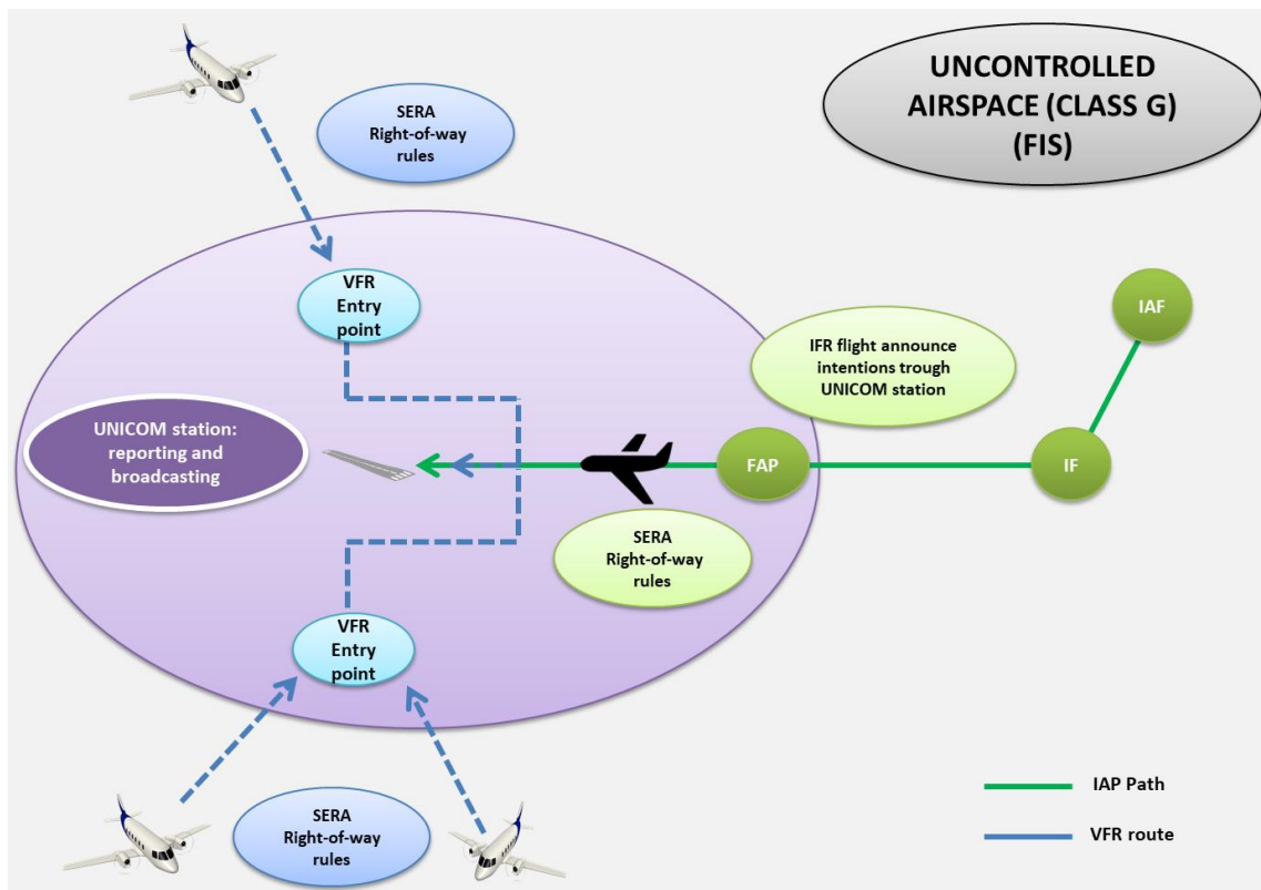
Figure 15: IFR/VFR integration in an aerodrome with non-ATS aeronautical stations: UNICOM (plan view)
