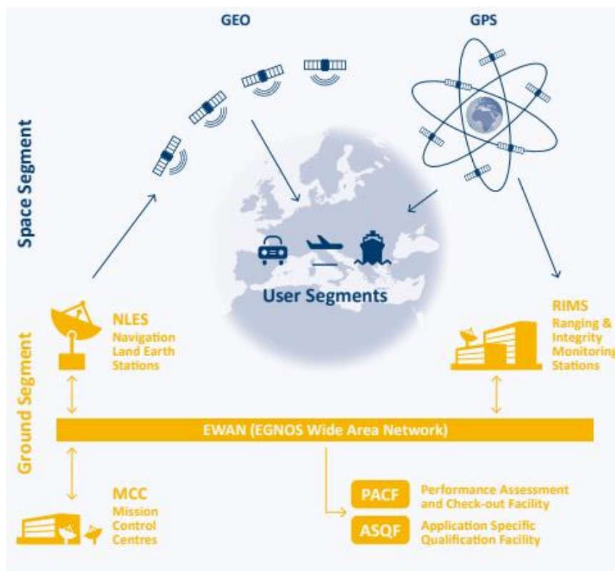
Figure 6: EGNOS architecture (source: EGNOS SDD [RD-11])
