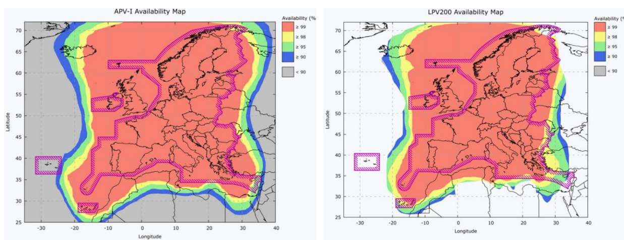
Figure 5: APV-I and LPV-200 Availability Map (source: EGNOS SDD [RD-11])
